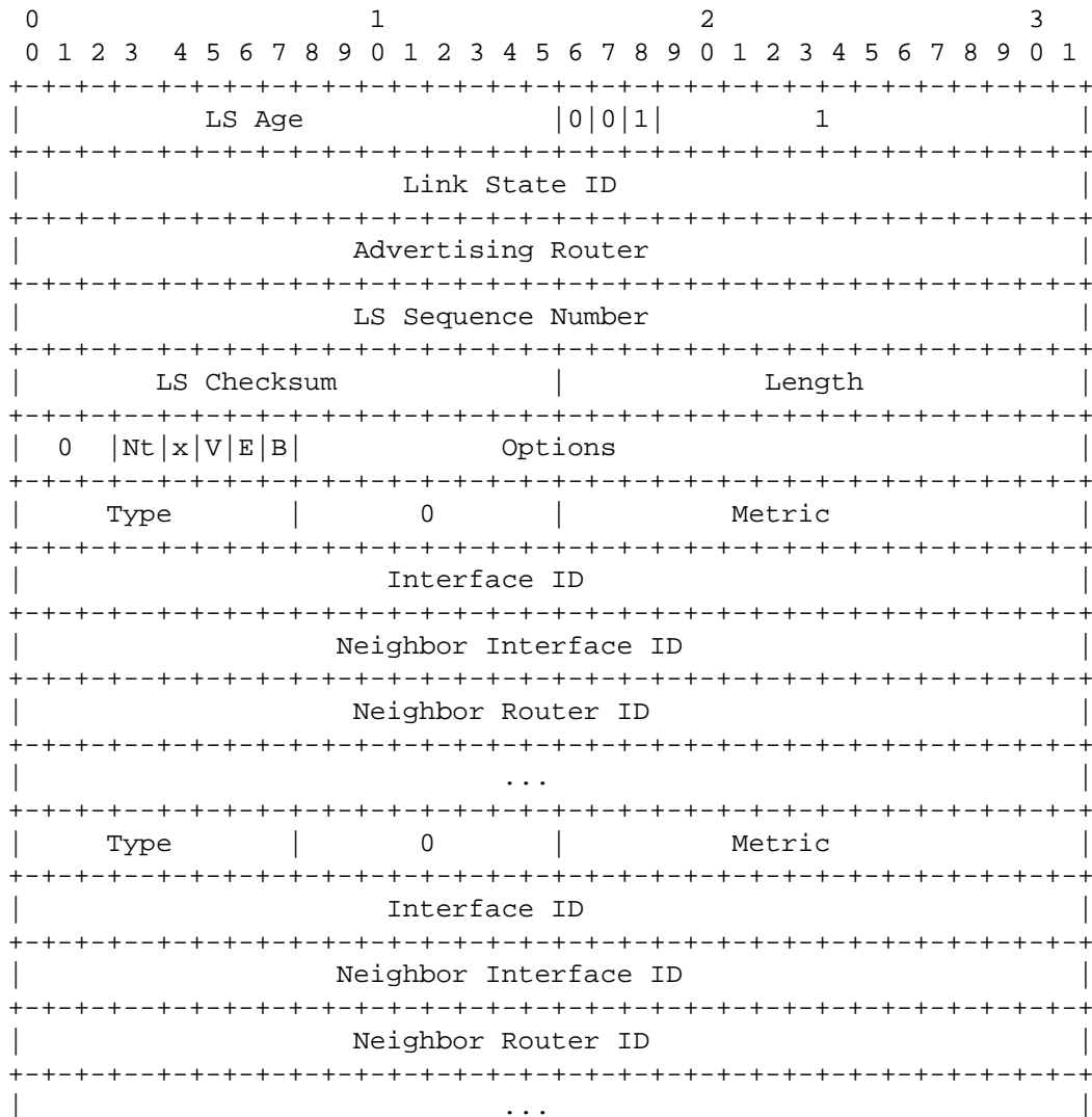
Router-LSA Format
