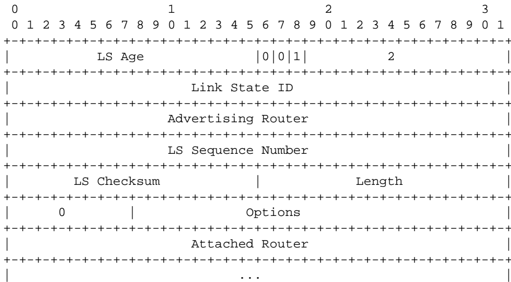
Network-LSA Format
