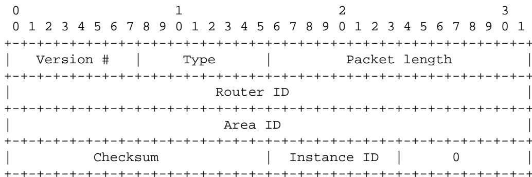
The OSPF Packet Header
