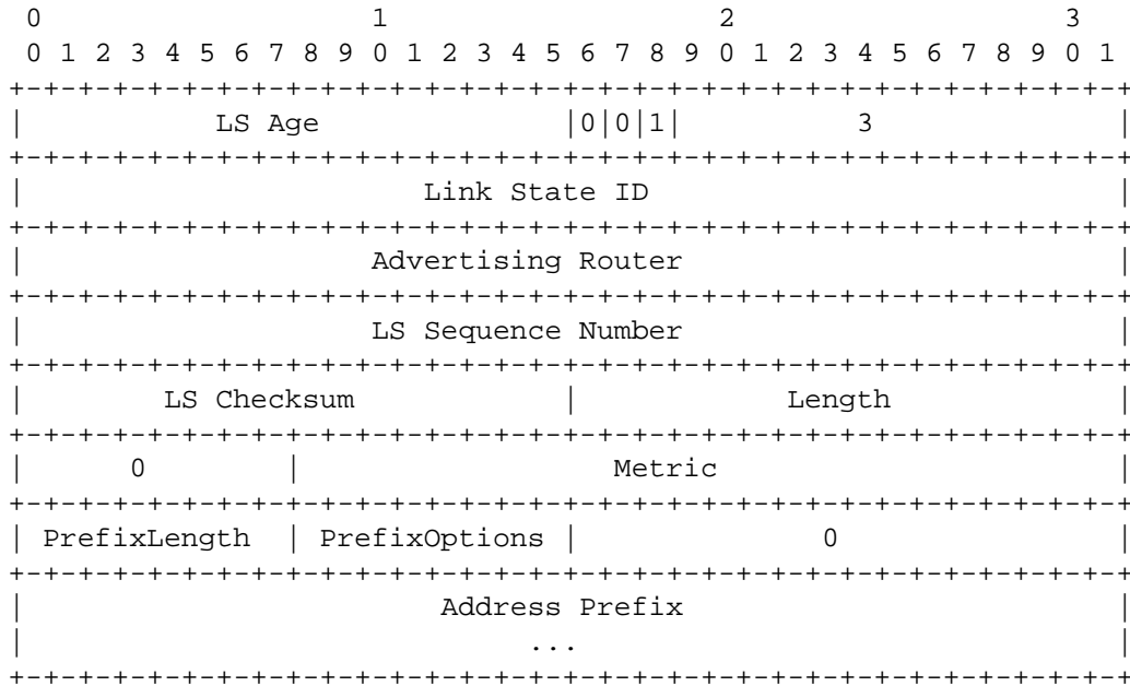
Inter-Area-Prefix-LSA Format
